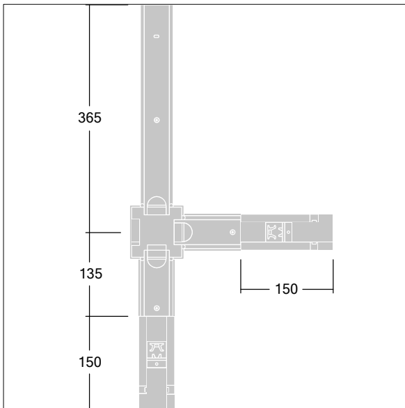
TL_CONTUS_M_T2_Node_Connector.wmf
